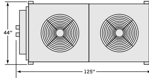
REMOTE CONDENSER (VERTICAL AIR FLOW)
